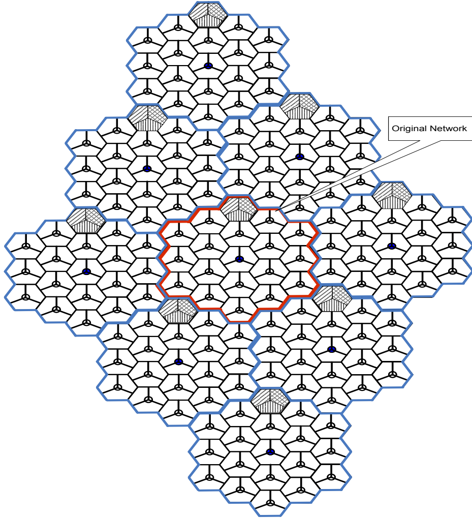
Figure 3: An example of wraparound network.
