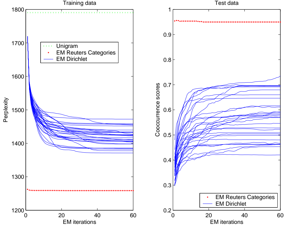
Figure 3: Evolution of Perplexity and Cooccurrence scores over the EM iterations for different Dirichlet initializations for the first fold.
