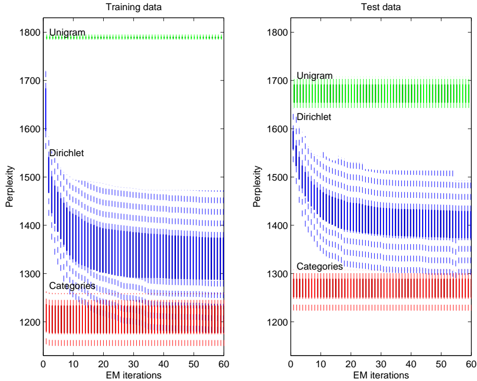
Figure 2: Evolution of Perplexity on training and test data over the EM iterations.
