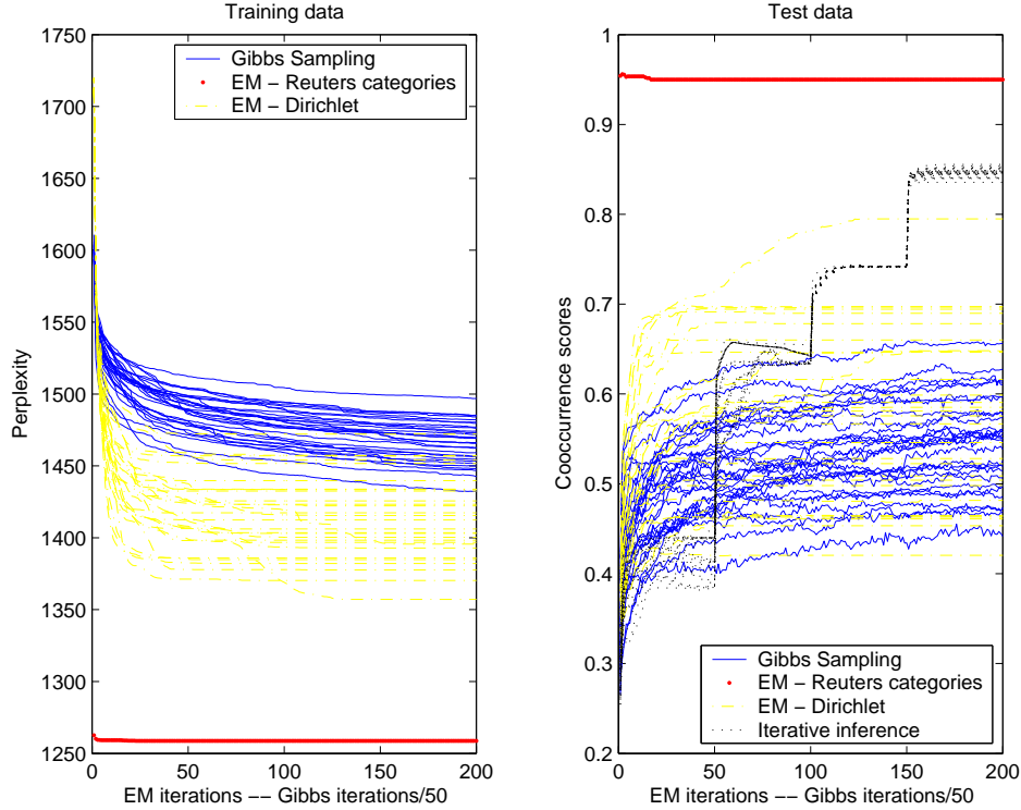
Figure 10: Evolution of perplexity and cooccurrence scores over the EM-Gibbs Sampling iterations.
